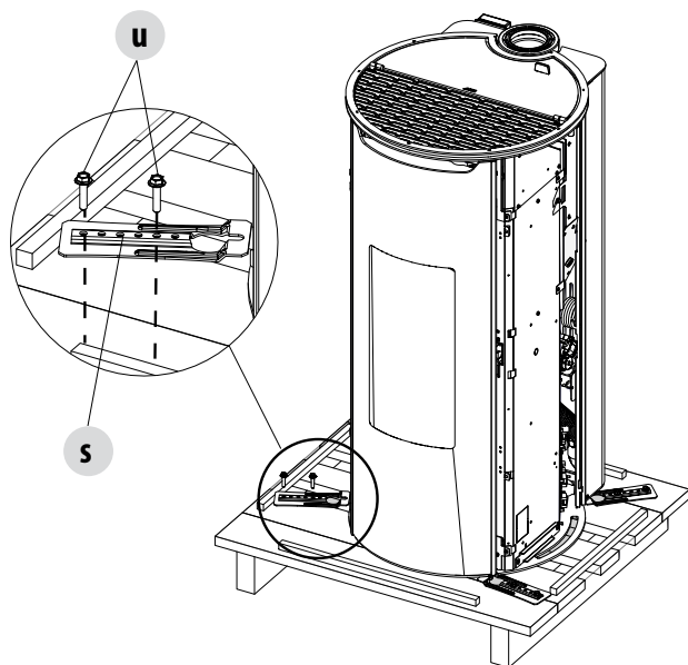
REMOVING THE FASTENING BRACKETS
