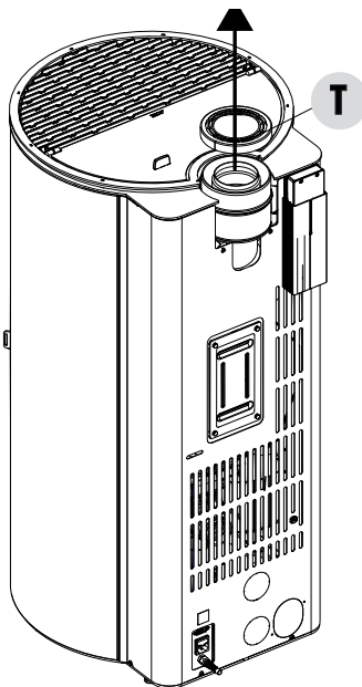
INSTALLATION TYPE "XUP" DOUBLE-WALL SMOKE OUTLET
